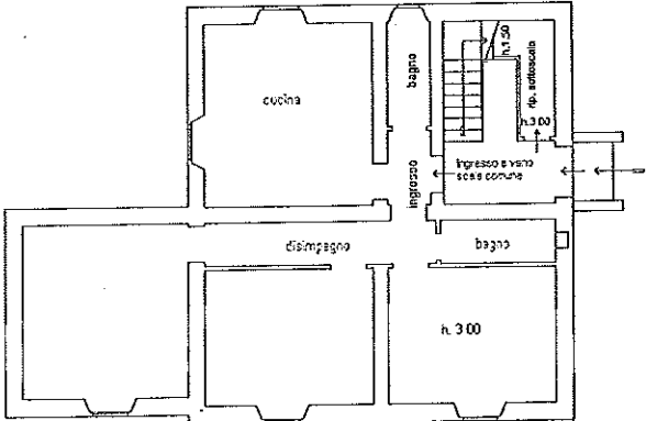
PIANO TERRENO
