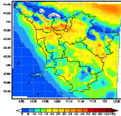
PM25 [ \mu\text{g}/\text{m}^3 ] MEDIA 11 2015
