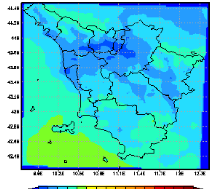
O3nopeak [ \mu\text{g}/\text{m}^3 ] MEDIA 11 2015
