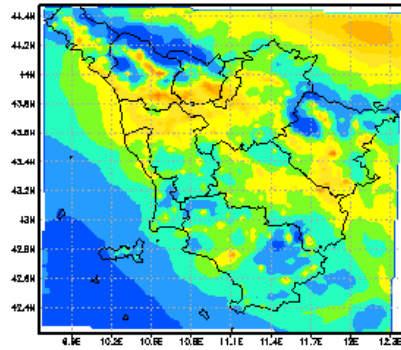
PM 10 [ \mu\text{g}/\text{m}^3 ] MEDIA INVERNO 2015
