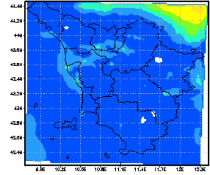
PM 25 [ \mu\text{g}/\text{m}^3 ] MEDIA ESTATE 2015
