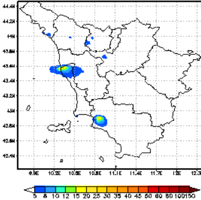
SO2 [ \mu\text{g}/\text{m}^3 ] MEDIA 11 2015
