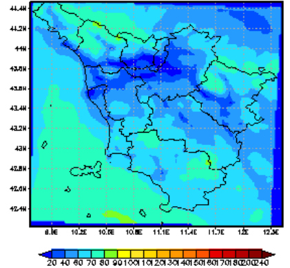
O3nopeak [ \mu\text{g}/\text{m}^3 ] MEDIA 11 2015
