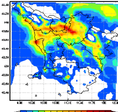
SO2 [ \mu\text{g}/\text{m}^3 ] MEDIA 11 2015
