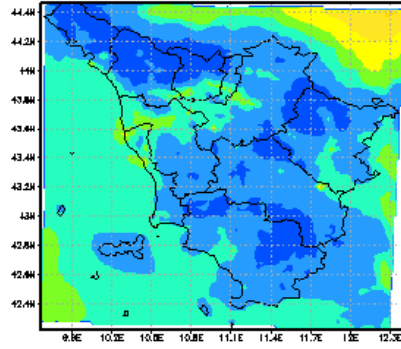
PM 10 [ \mu\text{g}/\text{m}^3 ] MEDIA ESTATE 2015
