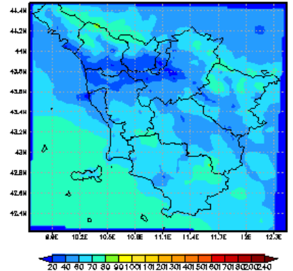
O3nopeak [ \mu\text{g}/\text{m}^3 ] MEDIA 12 2015
