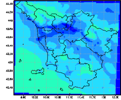
O 3 [ \mu\text{g}/\text{m}^3 ] MEDIA nopeak INVERNO 2015
