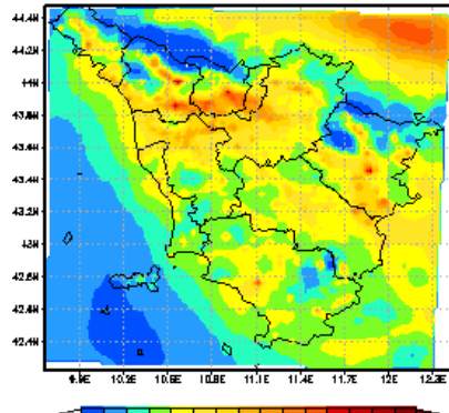
PM25 [ \mu\text{g}/\text{m}^3 ] MEDIA 11 2015
