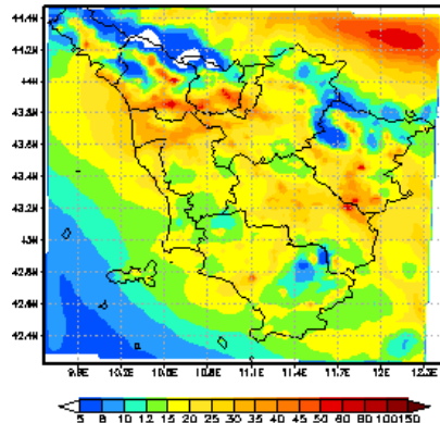
PM25 [ \mu\text{g}/\text{m}^3 ] MEDIA 12 2015
