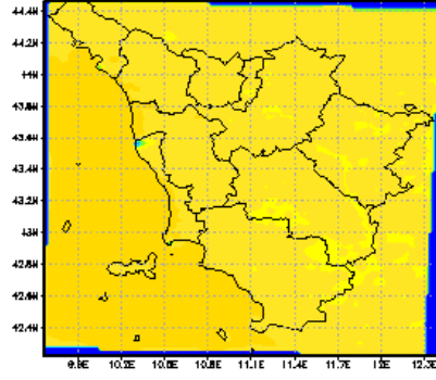
O 3 [ \mu\text{g}/\text{m}^3 ] MEDIA peak ESTATE 2015
