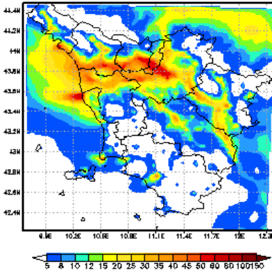
SO2 [ \mu\text{g}/\text{m}^3 ] MEDIA 12 2015
